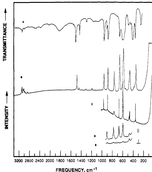
Figure 4. Vibrational spectra of \text{N}(\text{CH}_3)_4^+\text{IOF}_6^- . Trace A, infrared spectrum of the solid as an AgBr disk; traces B and C, Raman spectra of the solid at 25 and -146^\circ\text{C} ; traces D and E, Raman spectra of the \text{CH}_3\text{CN} solution with parallel and perpendicular polarization, respectively.
