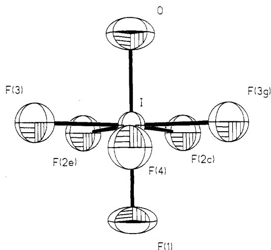
Figure 2. The structure of the IOF 6 - anion showing the puckering pattern of the equatorial fluorine ligands.
